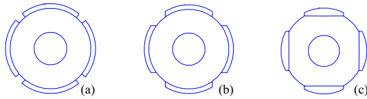
Fig. 1. Analyzed types of permanent magnet motors
