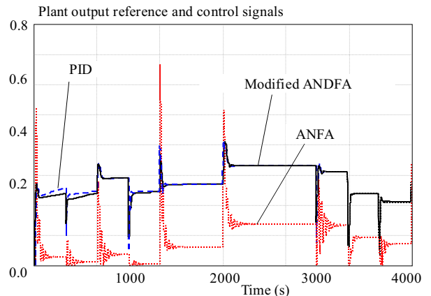
Fig. 8. Control signals of the PID, ANFA PID and Modified ANFA PID controllers
