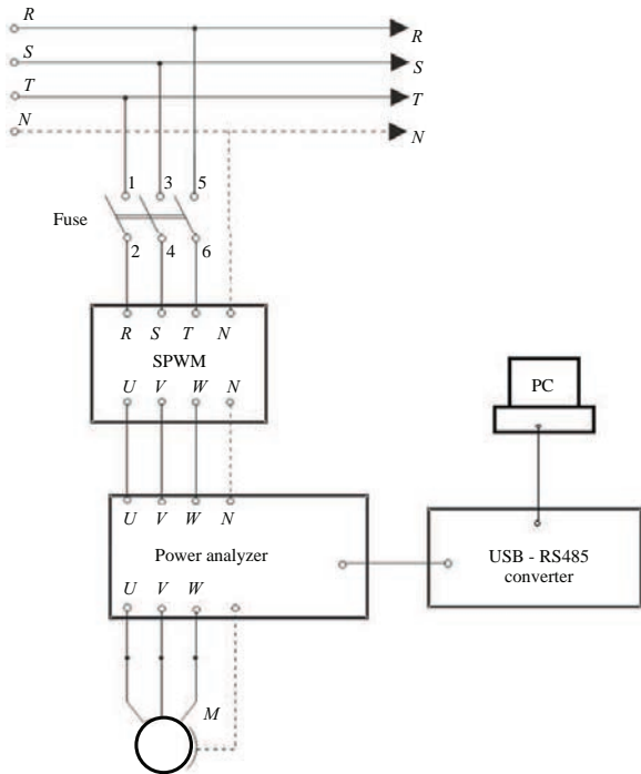
Fig. 1. IM connection diagram for experimental application
