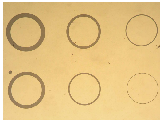
Fig. 1. Au/Ni-Mg /SWCNT/p-GaN contact structure for CTLM ohmic contact characterization. The outer radius of the test patterns is 155 \mu\text{m} with gap length from 5 to 45 \mu\text{m} .
