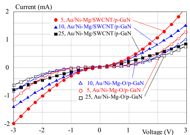
Fig. 2. I-V curves for gap length 5, 10 and 25 \mu\text{m} from CTLM measurements of Au/Ni-Mg/SWCNT/p-GaN contacts annealed in N_2 at 700 °C for 1 minute and of Au/Ni-Mg-O/p-GaN contacts annealed in N_2 at 500 °C for 2 minutes
